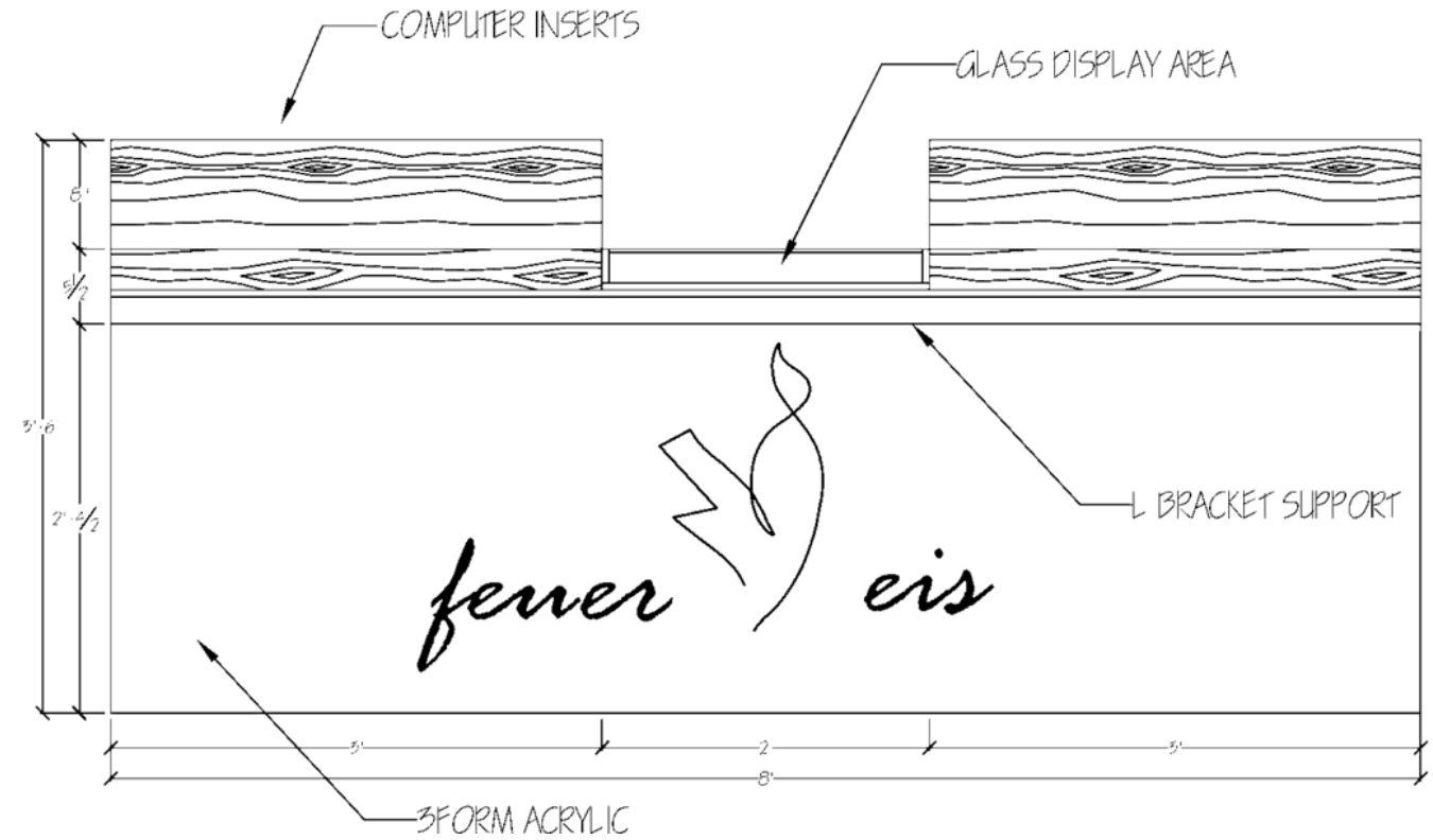
Front Bar: Front View
