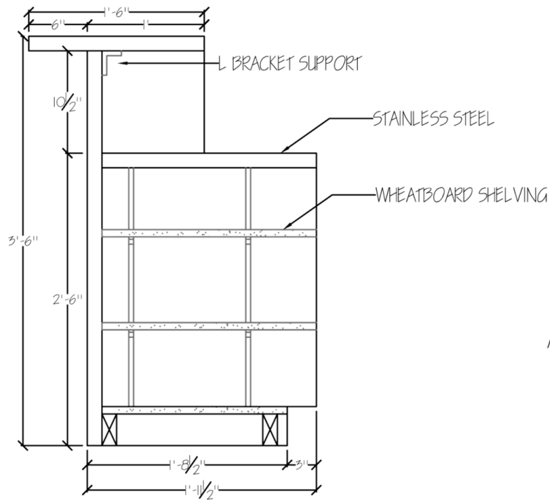
Front Bar: Section View
