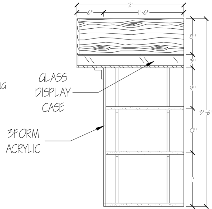
Host Stand: Side View
